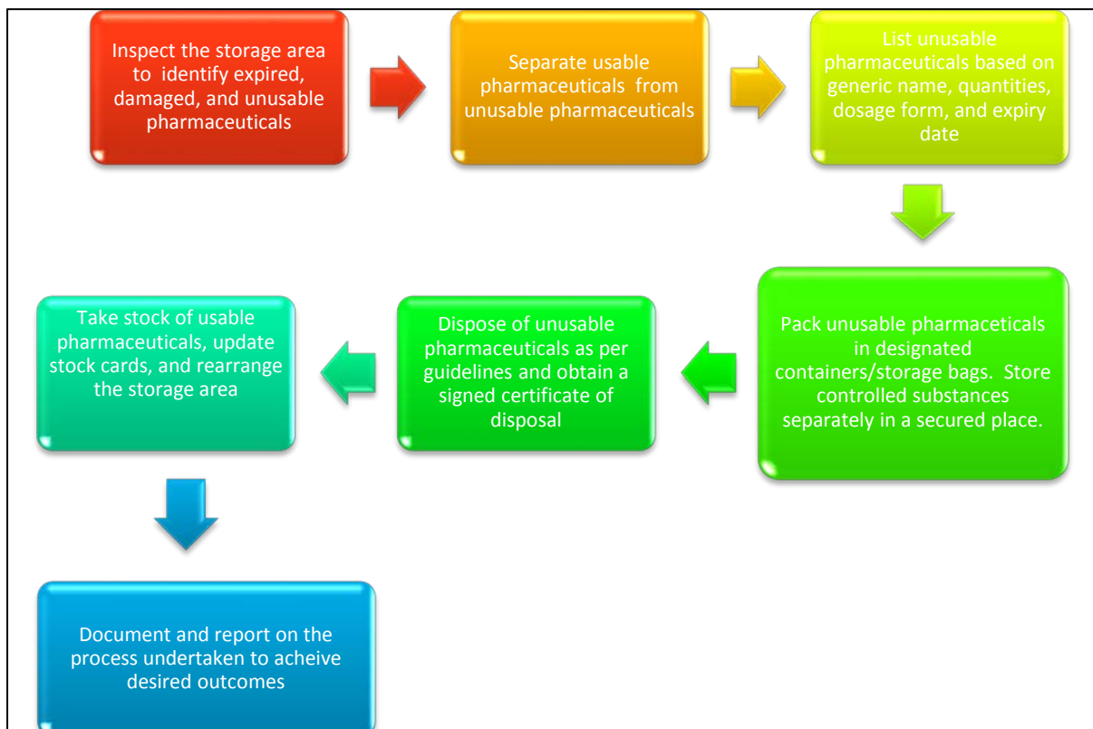
Figure 1. Step by step tasks for de-junking
