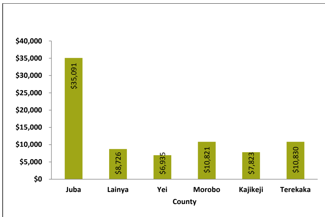
Figure 2. Value of de-junked pharmaceuticals in CES
